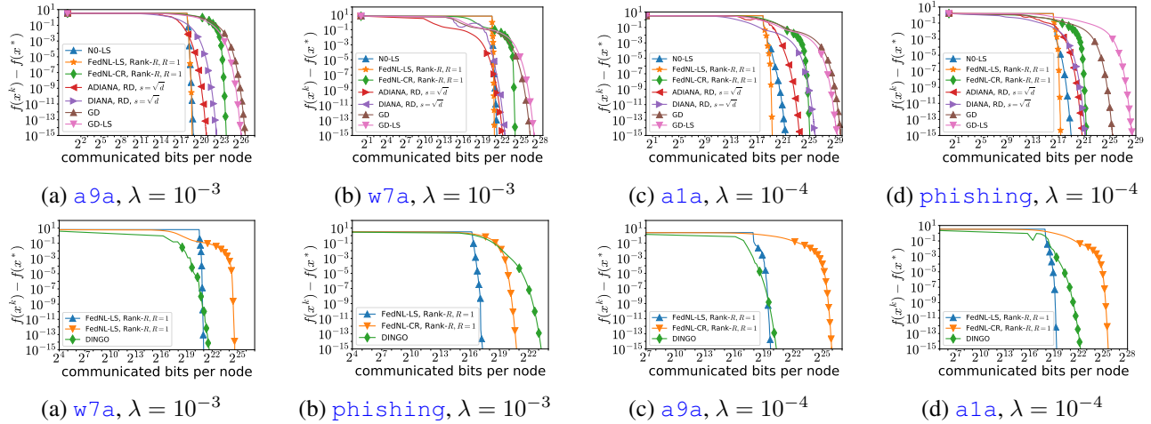
Figure 13. First row: Global comparison of FedNL-LS, NO-LS, and FedNL-CR with ADIANA, DIANA, GD, and GD-LS in terms of communication complexity. Second row: Global comparison of FedNL-LS and FedNL-CR with DINGO in terms of communication complexity.
