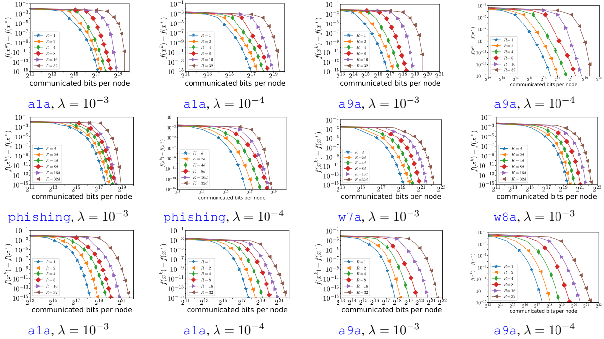
Figure 3. The performance of FedNL with different types of compression operators: Rank- R (first row); Top- K (second row); PowerSGD of rank R (third row) for several values of R and K in terms of communication complexity.
