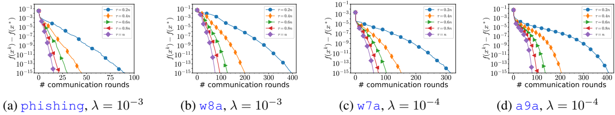
Figure 9. The performance of FedNL-PP with Rank-1 compressor in terms of iteration complexity.
