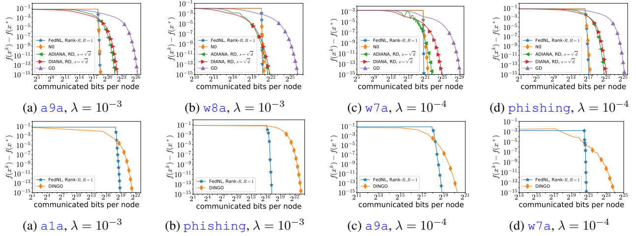
Figure 12. First row: Local comparison of FedNL and NO with ADIANA, DIANA, and GD in terms of communication complexity. Second row: Local comparison of FedNL with DINGO (second row) in terms of communication complexity.
