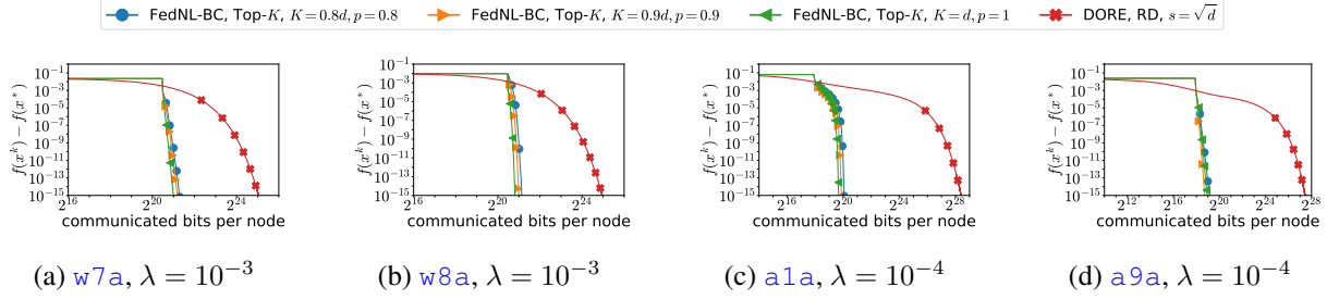
Figure 8. Comparison of FedNL-BC with Top- K applied to Hessians and models ( K = pd ), and broadcasting gradients with probability p and DORE in terms of communication complexity.
