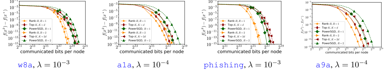
Figure 5. Comparison of the performance of FedNL with different compression operators in terms of communication complexity.
