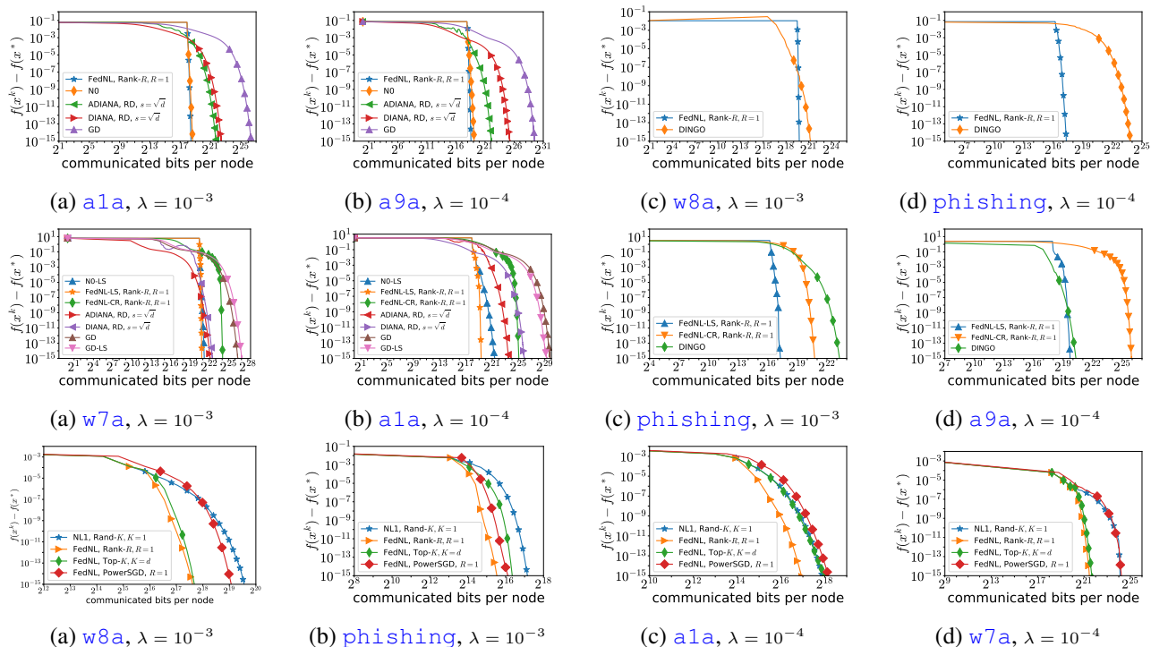
Figure 2. First row: Local comparison of FedNL and NO with (a), (b) ADIANA, DIANA, GD; with (c), (d) DINGO in terms of communication complexity. Second row: Global comparison of FedNL-LS, NO-LS and FedNL-CR with (a), (b) ADIANA, DIANA, GD, and GD with line search; with (c), (d) DINGO in terms of communication complexity. Third row: Local comparison of FedNL with 3 types of compression operators and NL1 in terms of communication complexity.
