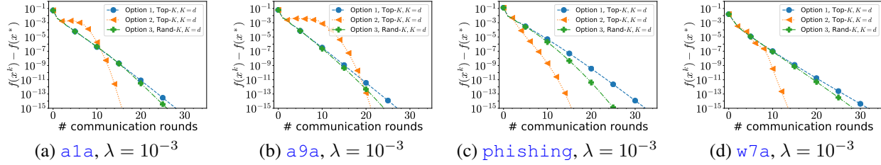
Figure 6. Comparison of FedNL with three update rules: Top- K , \alpha = 1 - \sqrt{1 - \delta} (Option 1); Top- K , \alpha = 1 (Option 2); Rand- K , \alpha = \frac{1}{\omega+1} (Option 3) in terms of iteration complexity.
