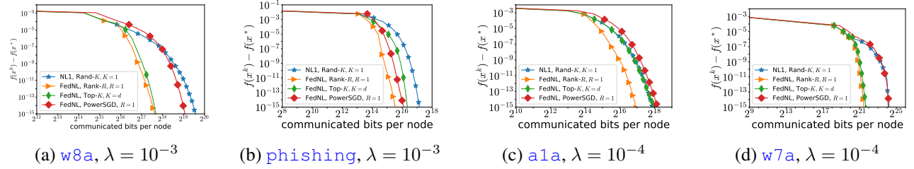
Figure 11. Comparison of FedNL with three types of compression and NL1 in terms of communication complexity.
