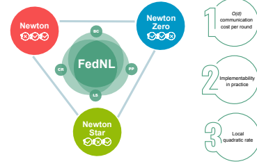
Figure 1. Visualization of the three special Newton-type methods—Newton (N), Newton Star (NS) and Newton Zero (NO)—as the vertices of a triangle capturing a subset of two of these three requirements: 1) \mathcal{O}(d) communication cost per round, 2) implementability in practice, and 3) local quadratic rate. Indeed, each of these three methods satisfies two of these requirements only: N (2+3), NS (1+3) and NO (1+2). Finally, the proposed FedNL framework with its four extensions to Partial Participation (FedNL-PP), globalization via Line Search (FedNL-LS), globalization via Cubic Regularization (FedNL-CR) and Bidirectional Compression (FedNL-BC) interpolates between these requirements.
