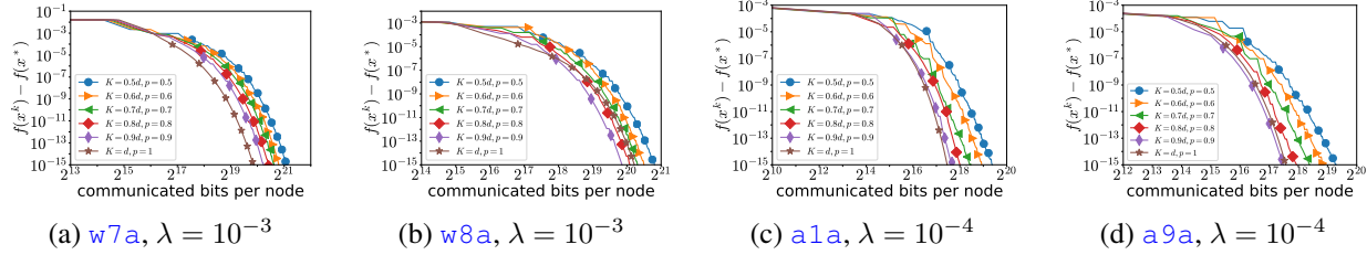
Figure 7. The performance of FedNL-BC with Top- K applied to Hessians and models ( K = pd ), and broadcasting gradients with probability p for several values of p in terms of communication complexity.
